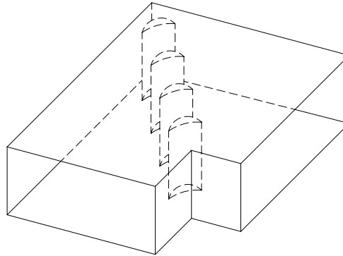
SQUARE THROAT & SQUARE BACK with TURNING VANES
